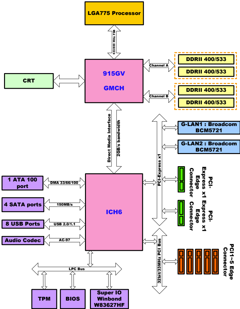
Figure 1.3: AIMB-760 Block Diagram
